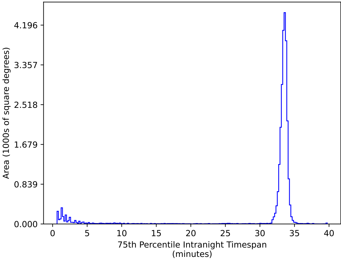
internal_u_expt30_nscale1.5v3.4_10yrs All sky ug bands: 75th Percentile Intranight Timespan
