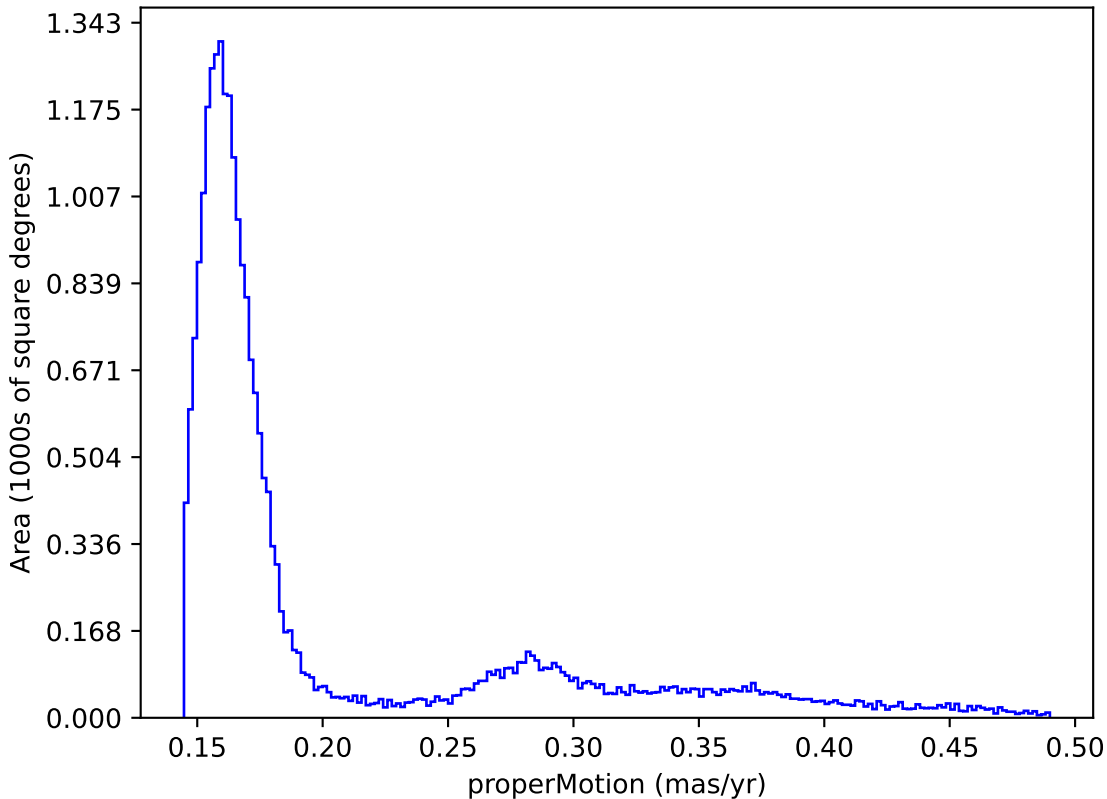
internal_u_expt30_nscale1.5v3.4_10yrs : properMotion
