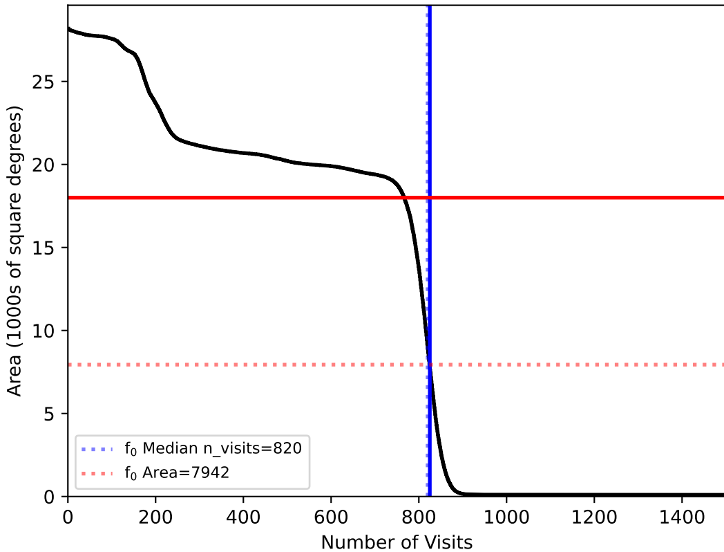
internal_u_expt30_nscale1.5v3.4_10yrs : fO
