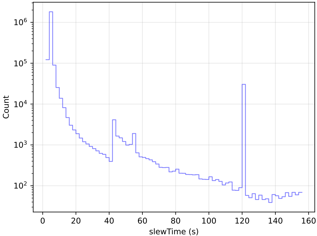
internal_u_expt30_nscale1.5v3.4_10yrs All visits: Slew Time Histogram
