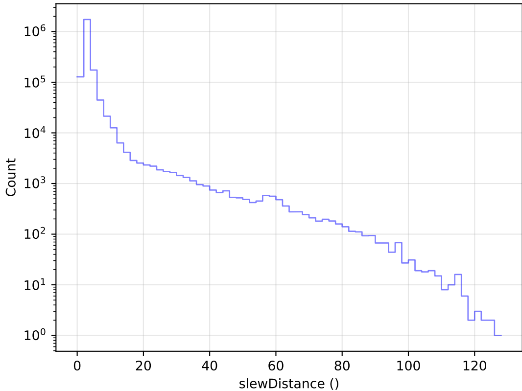
internal_u_expt30_nscale1.5v3.4_10yrs All visits: Slew Distance Histogram
