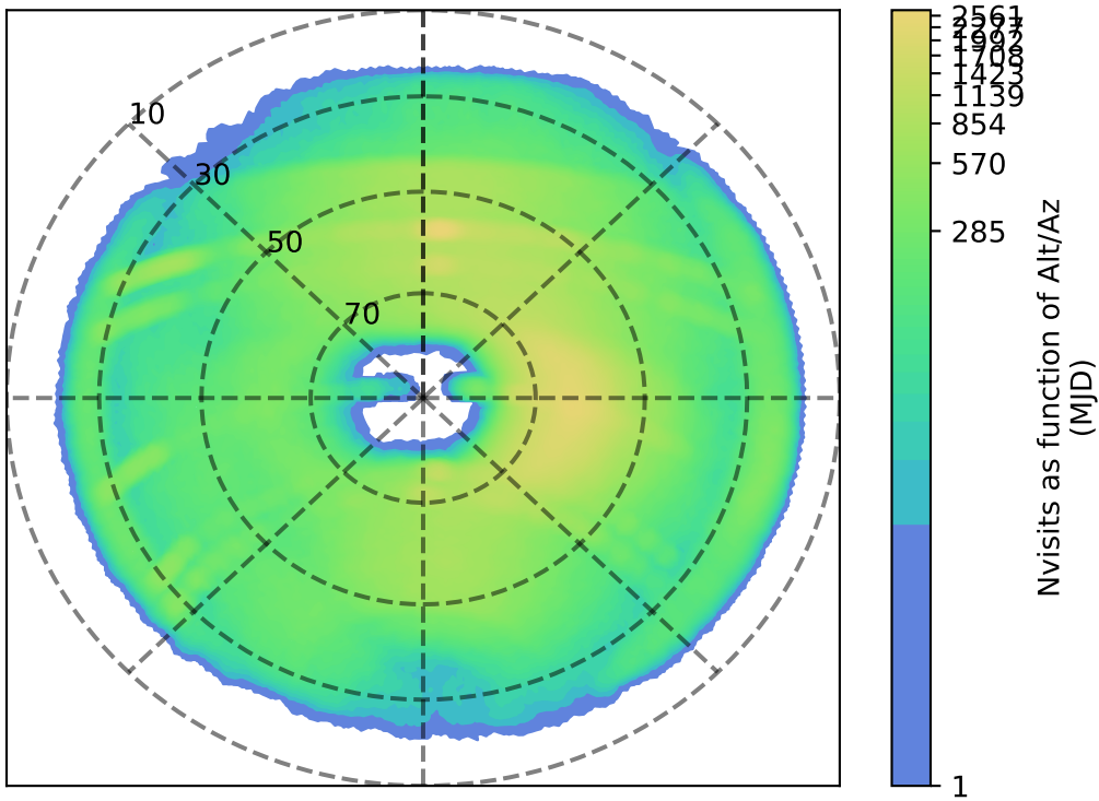
internal_u_expt30_nscale1.5v3.4_10yrs i: Nvisits as function of Alt/Az
