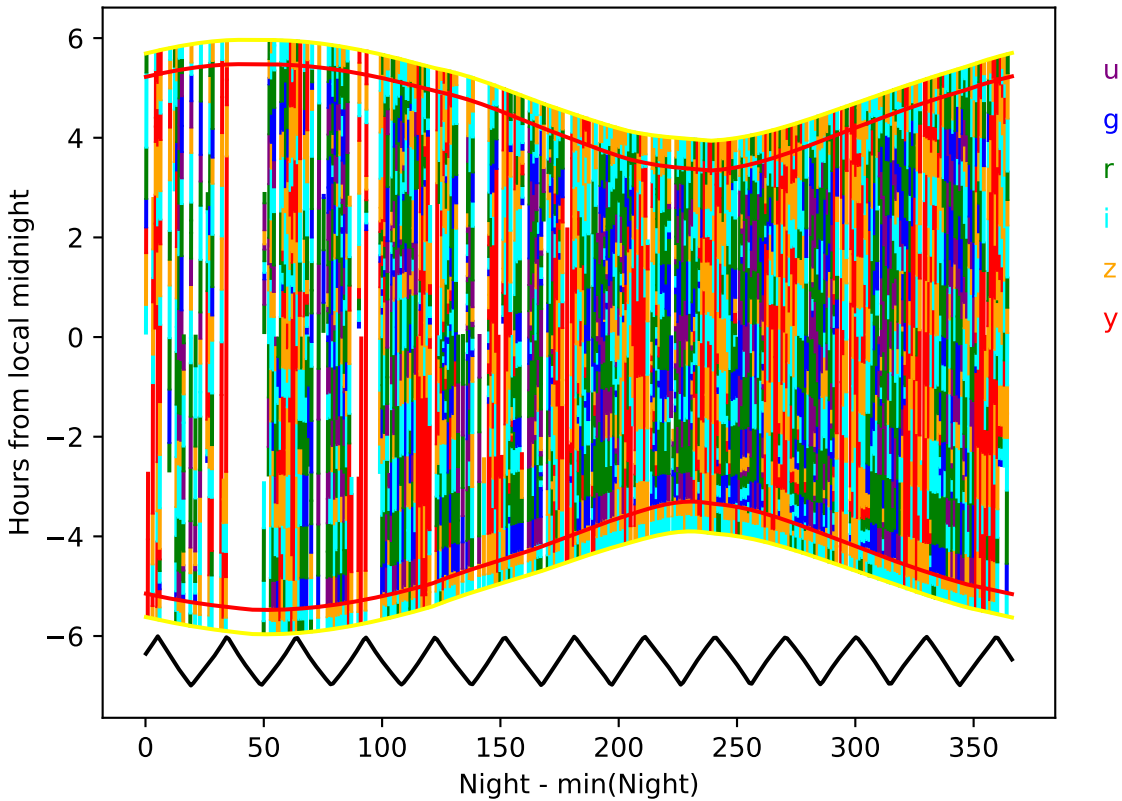
internal_u_expt30_nscale1.5v3.4_10yrs year 6-7: Hourglass
