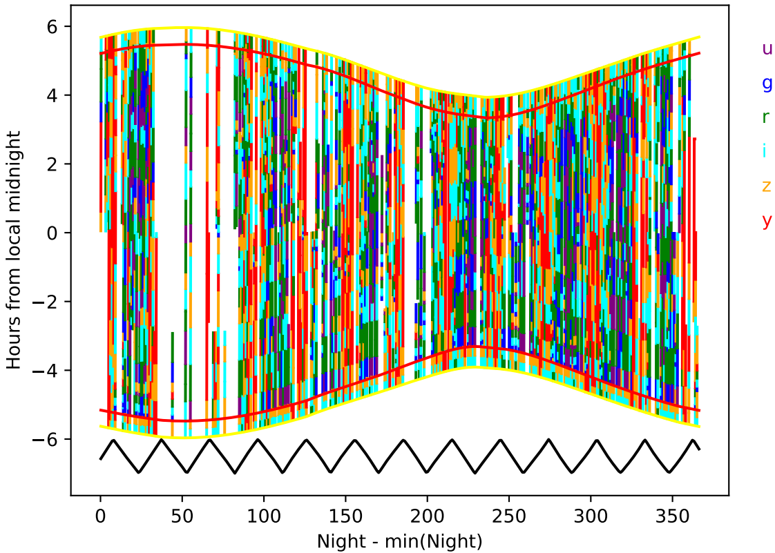
internal_u_expt30_nscale1.5v3.4_10yrs year 3-4: Hourglass
