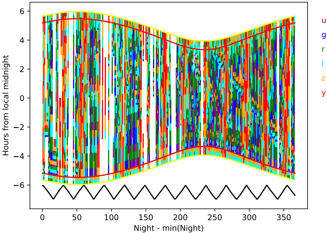
internal_u_expt30_nscale1.5v3.4_10yrs year 1-2: Hourglass
