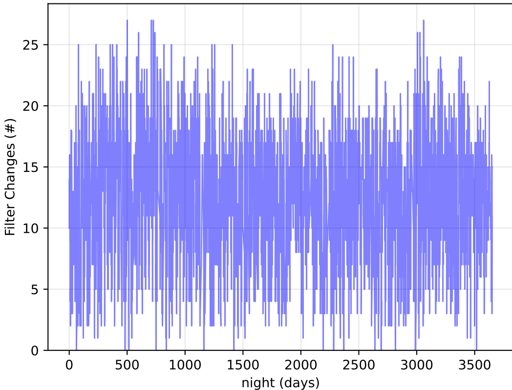
internal_u_expt30_nscale1.5v3.4_10yrs : Filter Changes
