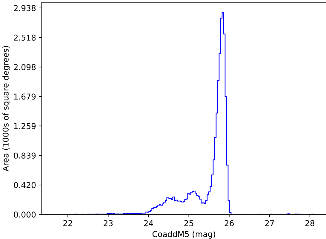
internal_u_expt30_nscale1.5v3.4_10yrs z: CoaddM5
