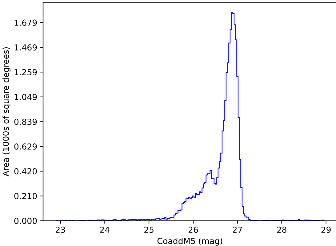
internal_u_expt30_nscale1.5v3.4_10yrs g: CoaddM5
