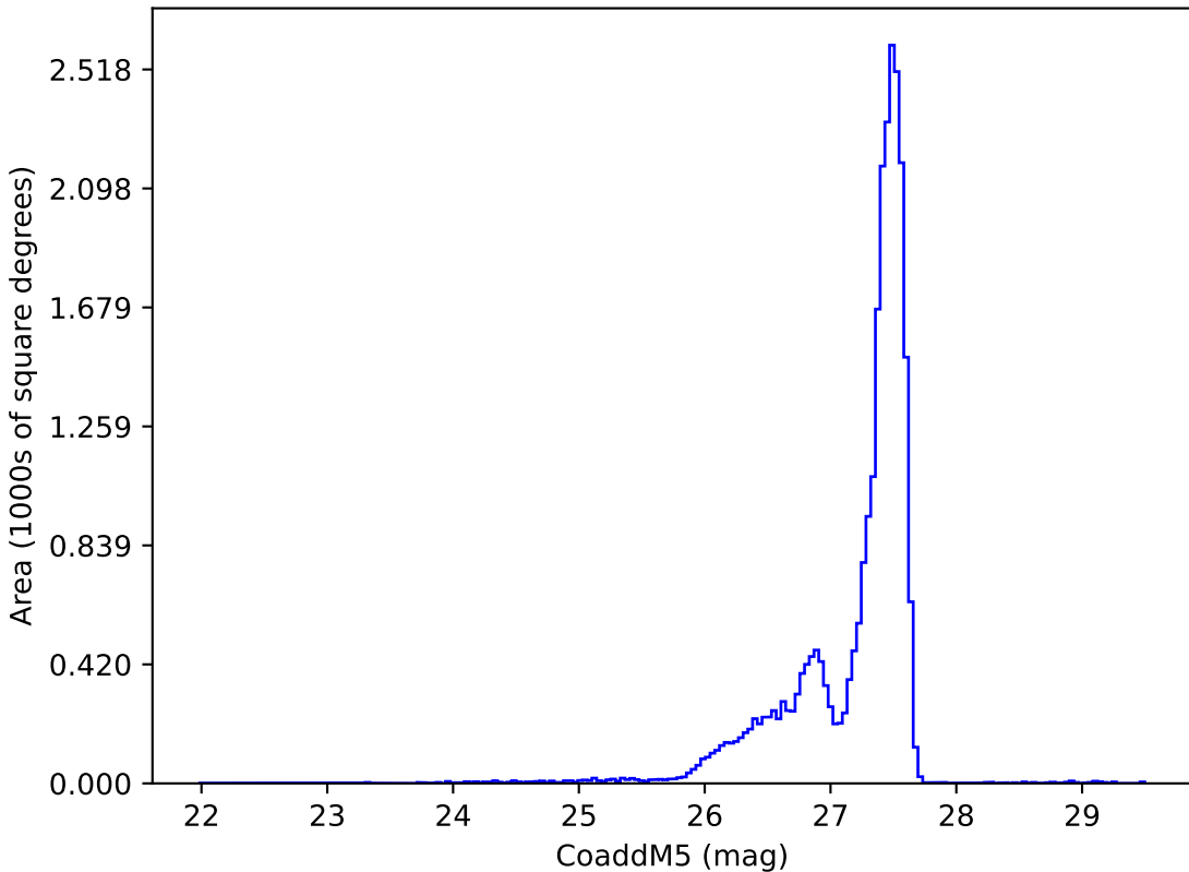
internal_u_expt30_nscale1.5v3.4_10yrs : CoaddM5
