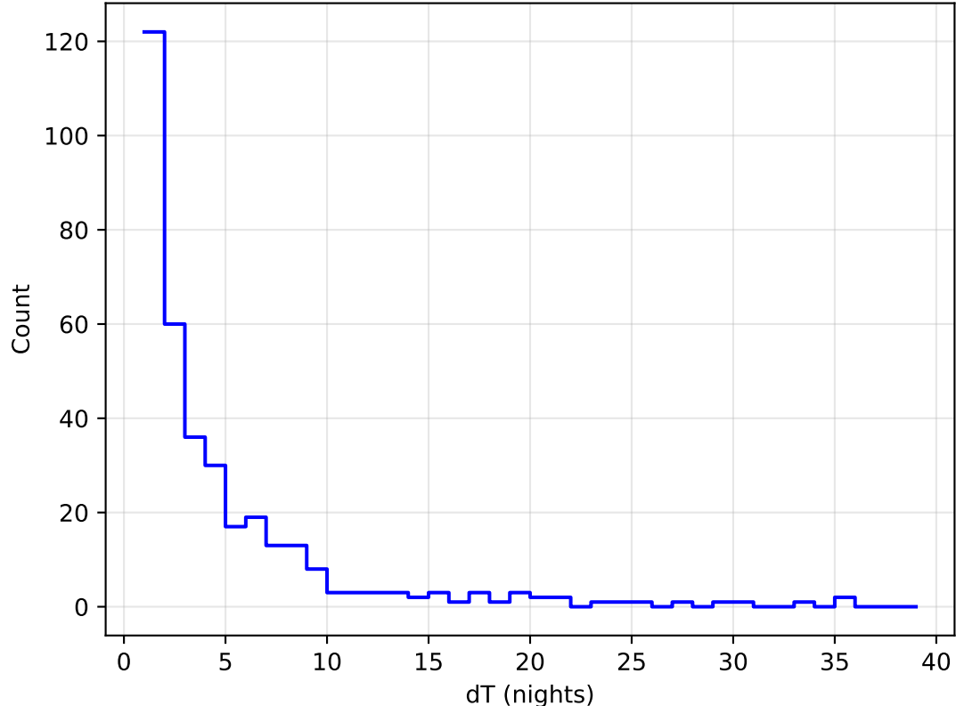
internal_u_expt30_nscale1.5v3.4_10yrs all bands: DD:WFD Delta Nights Histogram
