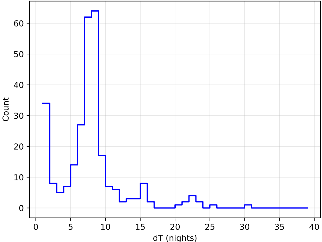
internal_u_expt30_nscale1.5v3.4_10yrs all bands: DD:ECDFS Delta Nights Histogram
