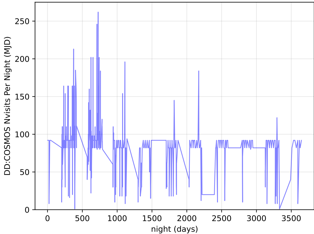
internal_u_expt30_nscale1.5v3.4_10yrs all bands: DD: COSMOS Nvisits Per Night
