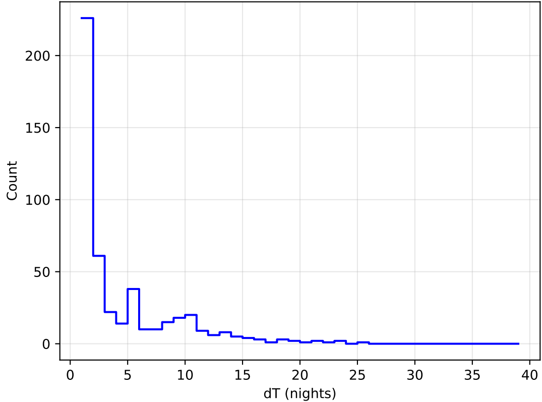
internal_u_expt30_nscale1.5v3.4_10yrs all bands: DD:COSMOS Delta Nights Histogram
