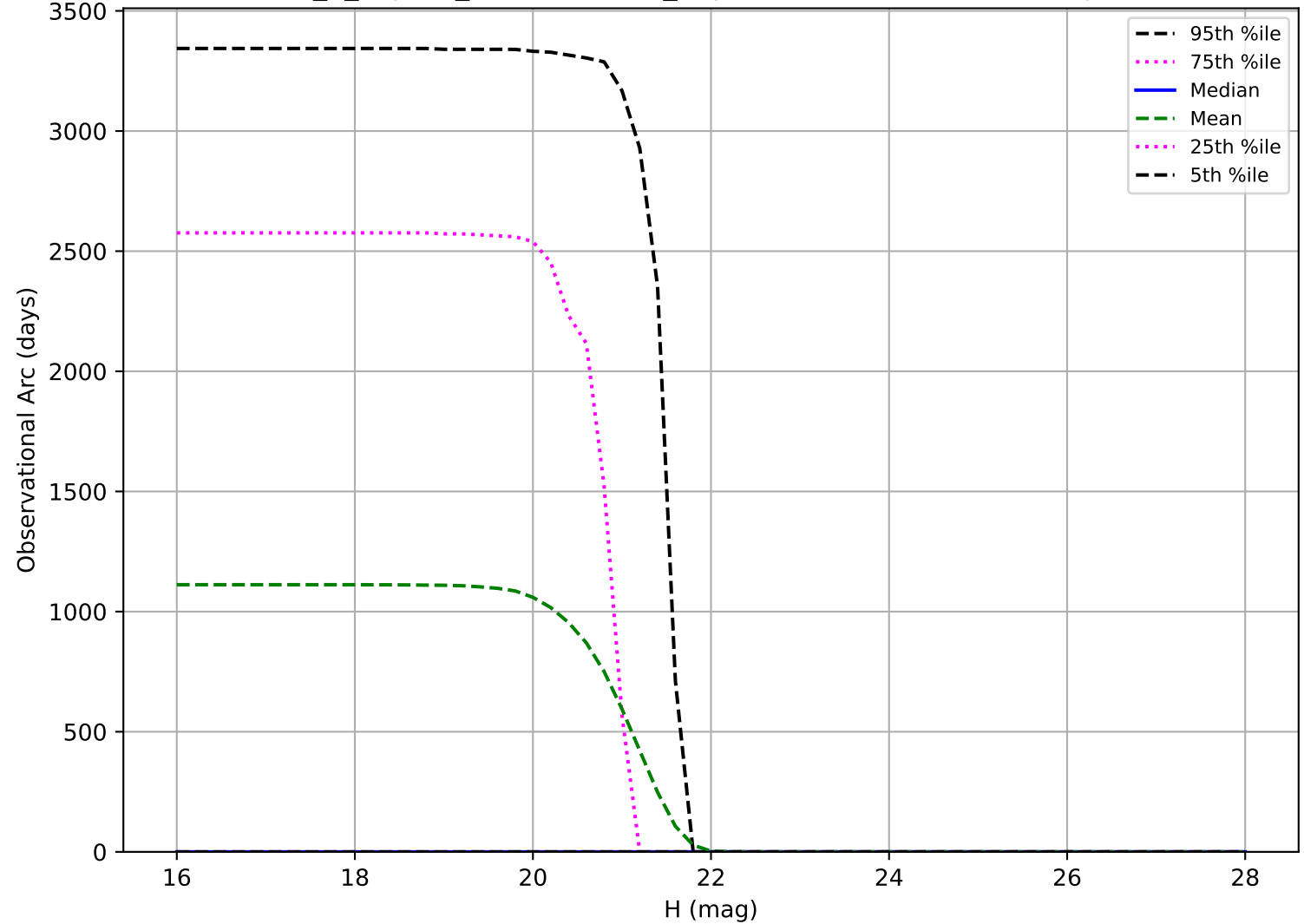
internal_u_expt30_nscale1.2v3.4_10yrs: Observational Arc Length Vatra
