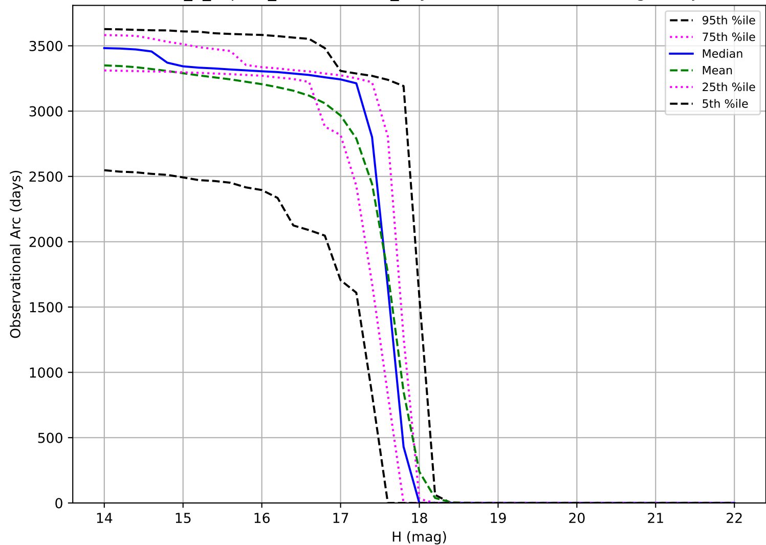
internal_u_expt30_nscale1.2v3.4_10yrs: Observational Arc Length Trojan
