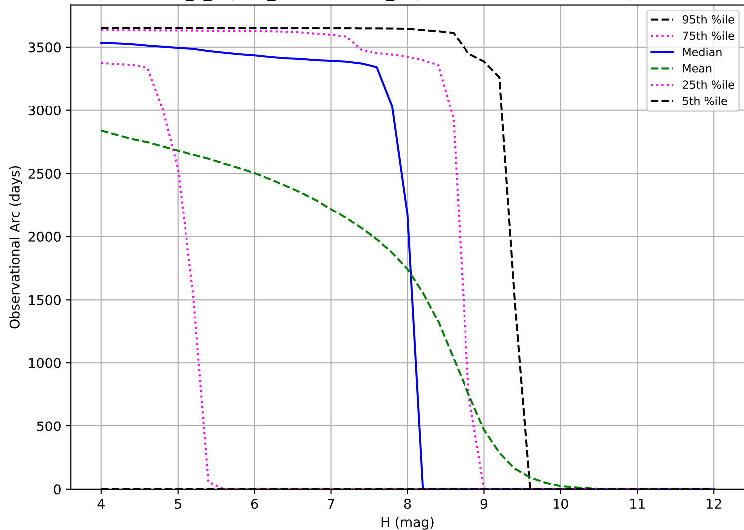
internal_u_expt30_nscale1.2v3.4_10yrs: Observational Arc Length TNO
