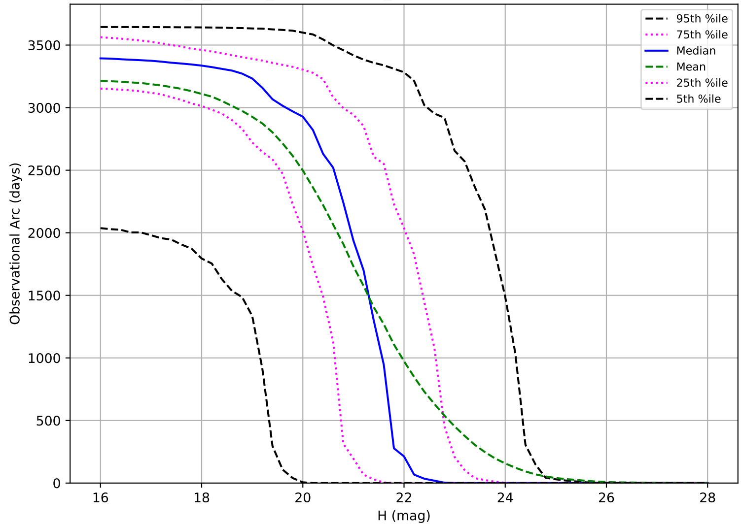
internal_u_expt30_nscale1.2v3.4_10yrs: Observational Arc Length PHA
