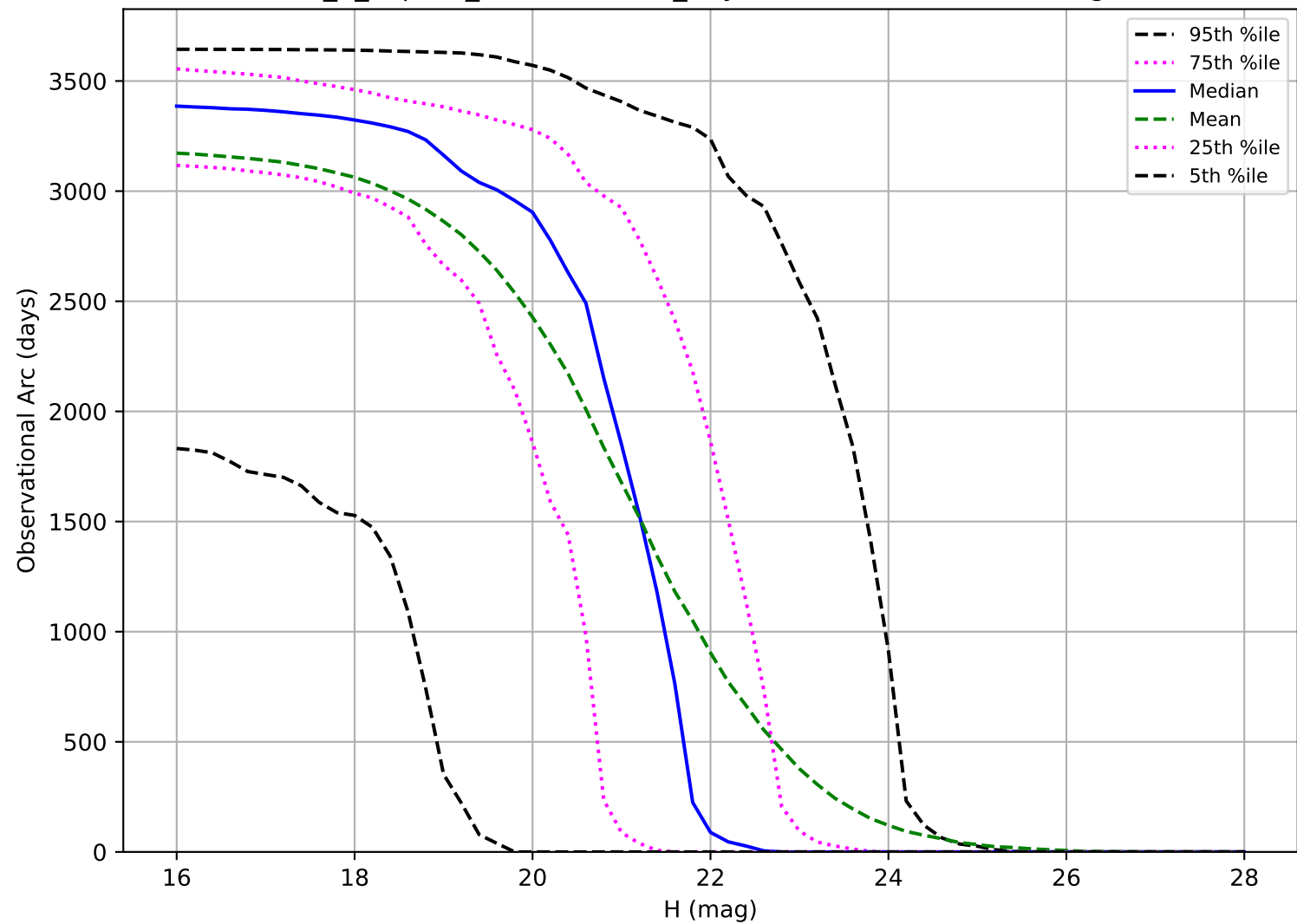
internal_u_expt30_nscale1.2v3.4_10yrs: Observational Arc Length NEO
