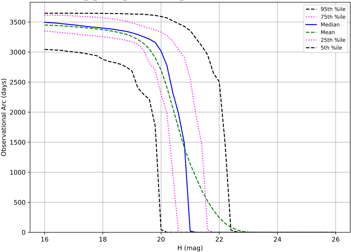
internal_u_expt30_nscale1.2v3.4_10yrs: Observational Arc Length MBA
