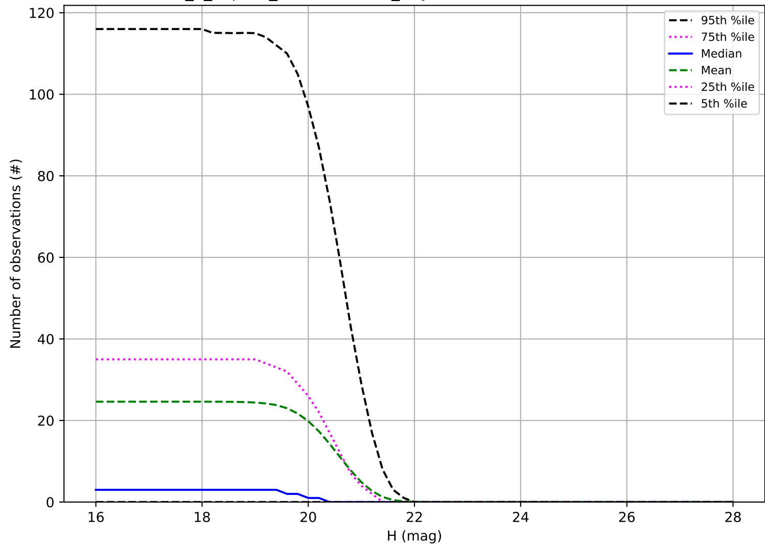
internal_u_expt30_nscale1.2v3.4_10yrs: Number of observations Vatira
