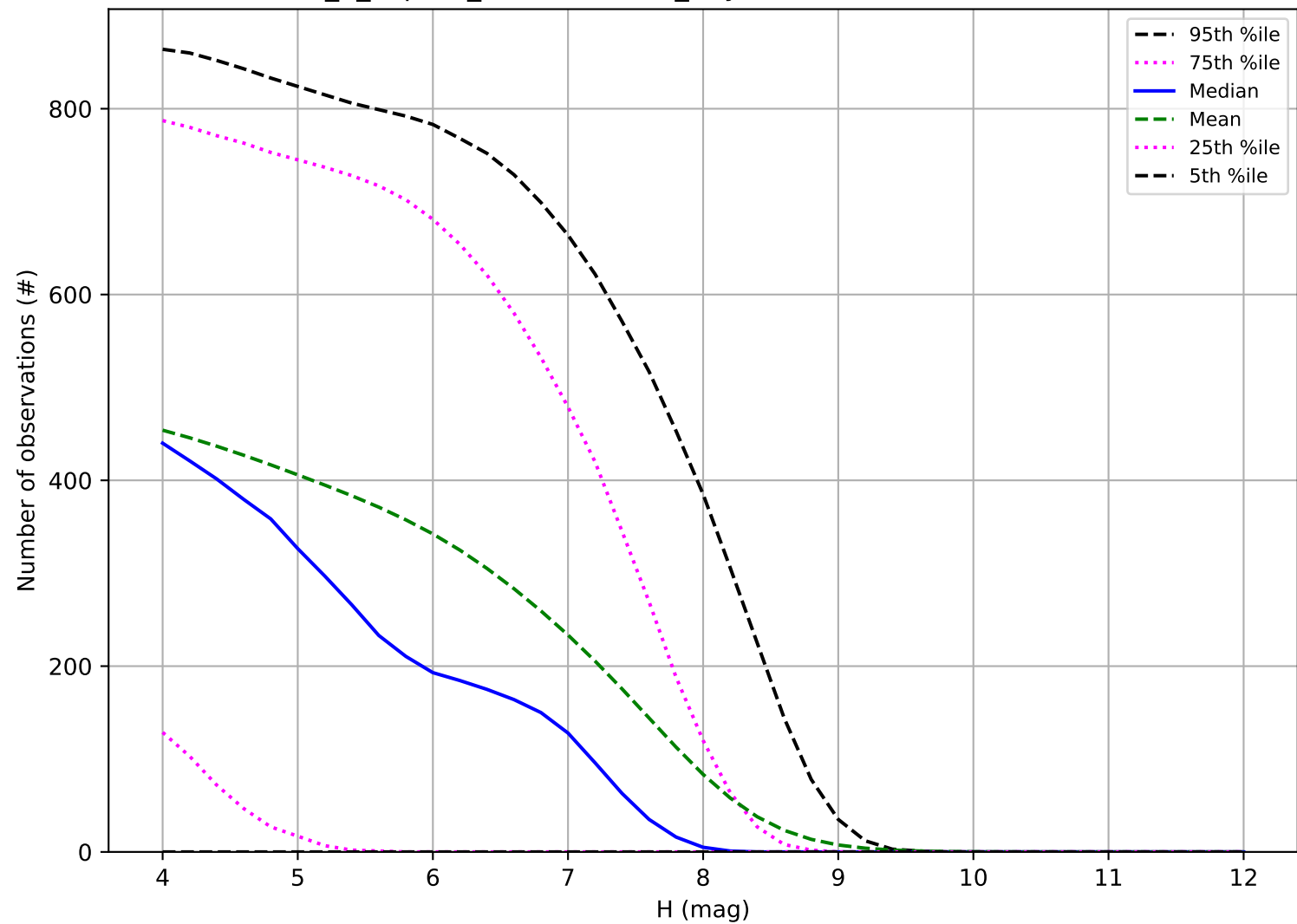
internal_u_expt30_nscale1.2v3.4_10yrs: Number of observations TNO
