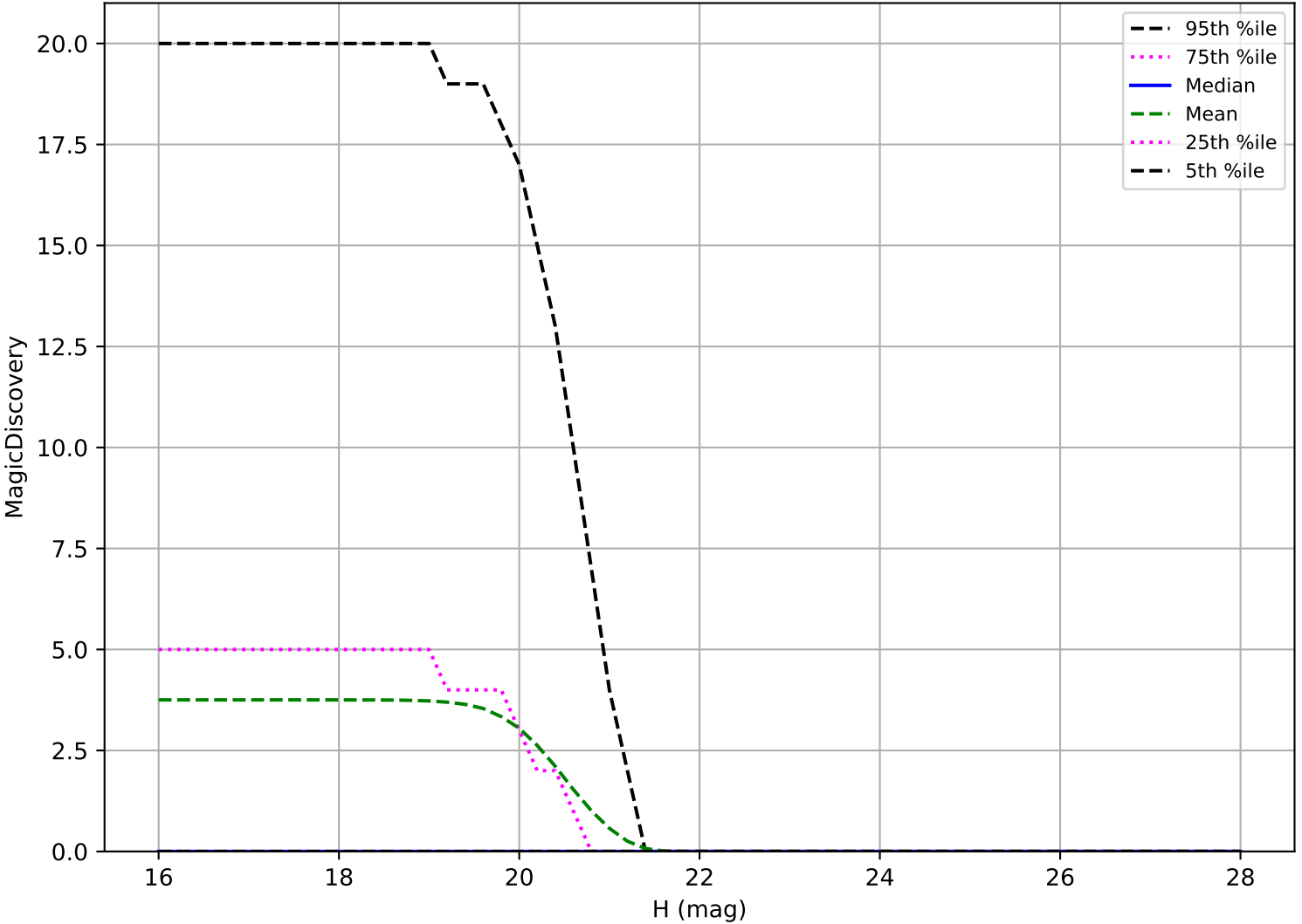
internal_u_expt30_nscale1.2v3.4_10yrs: Vatira 6 detections in 60 nights detection loss
