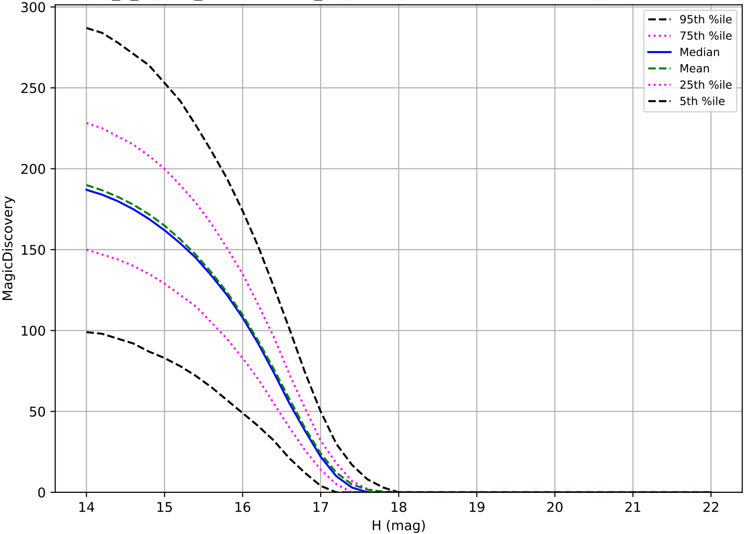
internal_u_expt30_nscale1.2v3.4_10yrs: Trojan 6 detections in 60 nights detection loss
