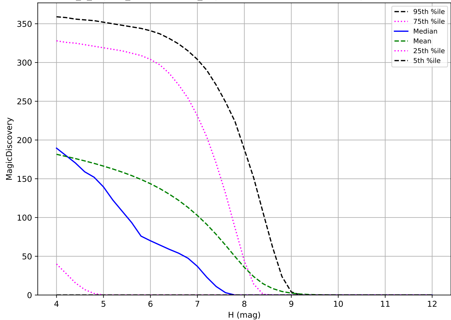
internal_u_expt30_nscale1.2v3.4_10yrs: TNO 6 detections in 60 nights detection loss
