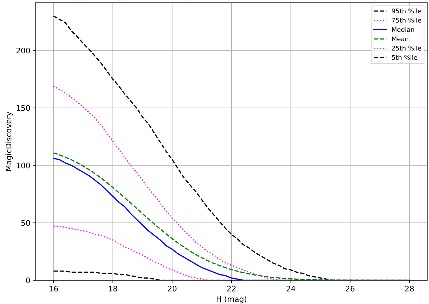
internal_u_expt30_nscale1.2v3.4_10yrs: PHA 6 detections in 60 nights detection loss
