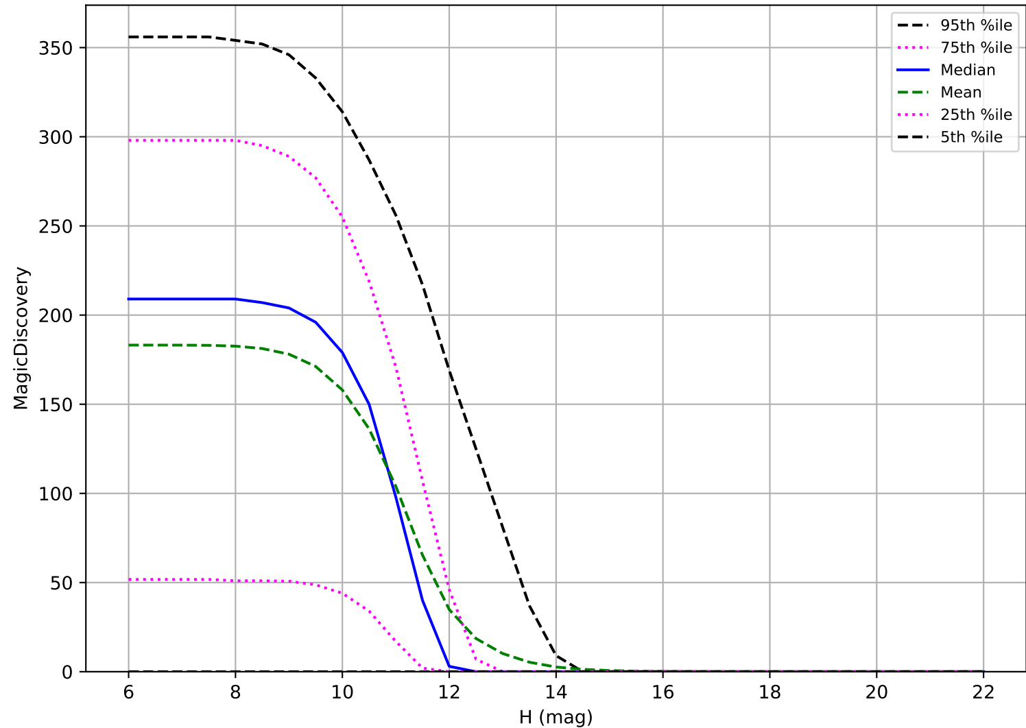
internal_u_expt30_nscale1.2v3.4_10yrs: OCC_r20 6 detections in 60 nights detection loss
