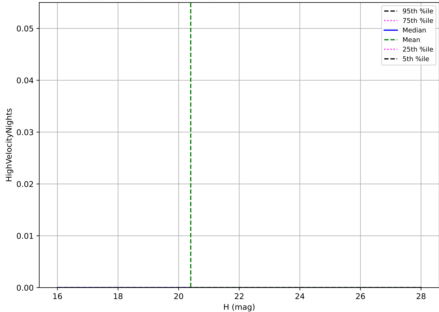
internal_u_expt30_nscale1.2v3.4_10yrs: Vatira High velocity pair detection loss
