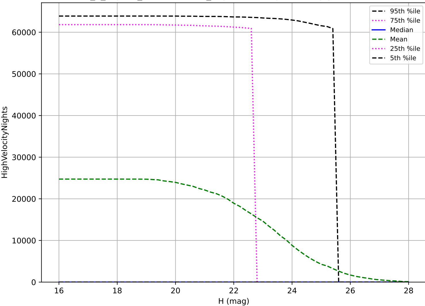
internal_u_expt30_nscale1.2v3.4_10yrs: PHA High velocity pair detection loss
