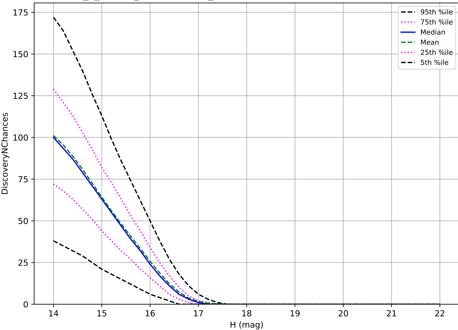
internal_u_expt30_nscale1.2v3.4_10yrs: Trojan 3 pairs in 15 nights detection loss
