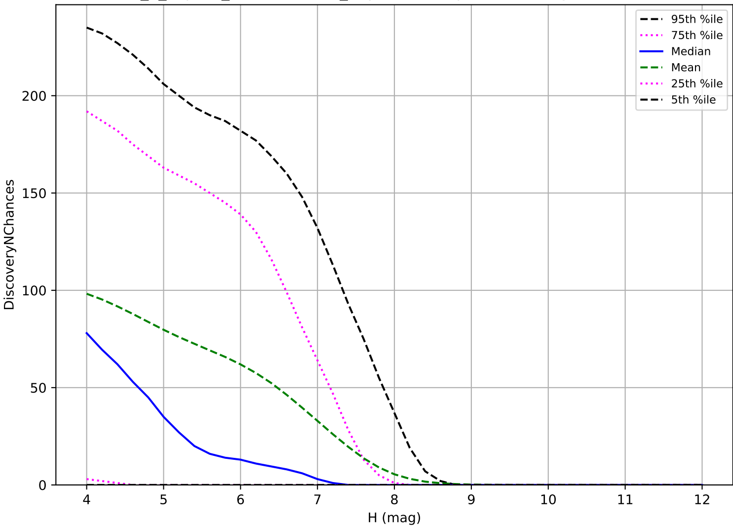
internal_u_expt30_nscale1.2v3.4_10yrs: TNO 3 pairs in 15 nights detection loss
