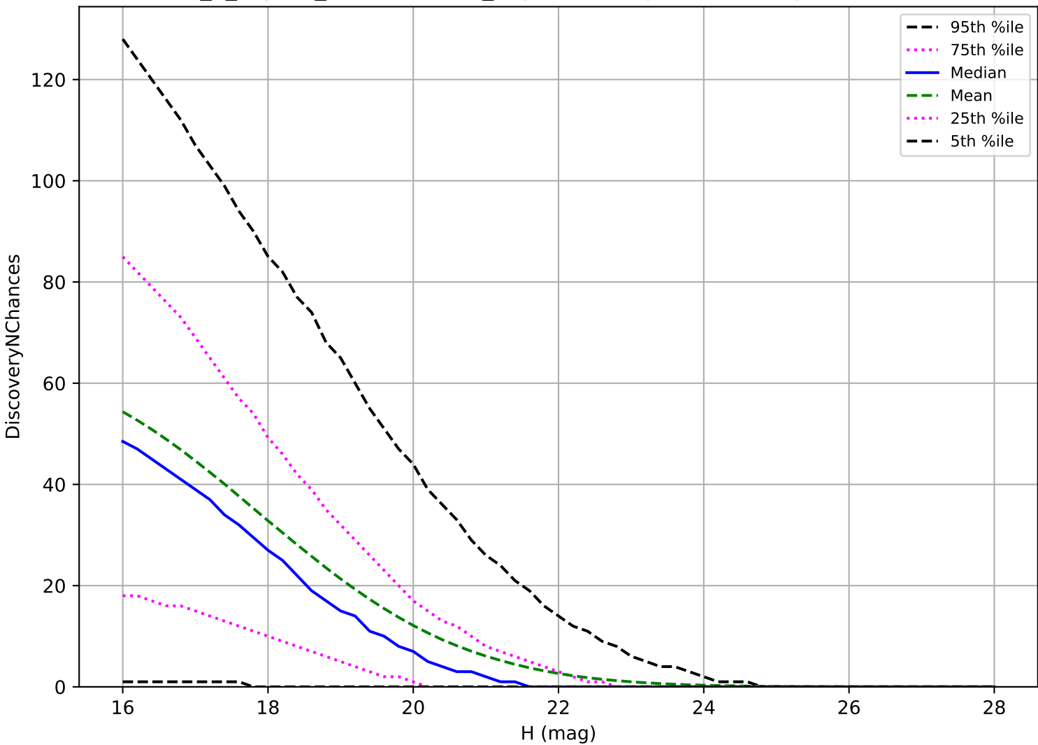
internal_u_expt30_nscale1.2v3.4_10yrs: PHA 3 pairs in 15 nights detection loss
