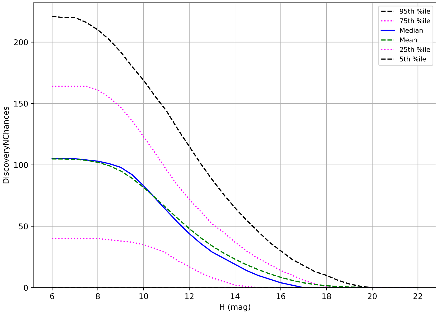
internal_u_expt30_nscale1.2v3.4_10yrs: OCC_r5 3 pairs in 15 nights detection loss
