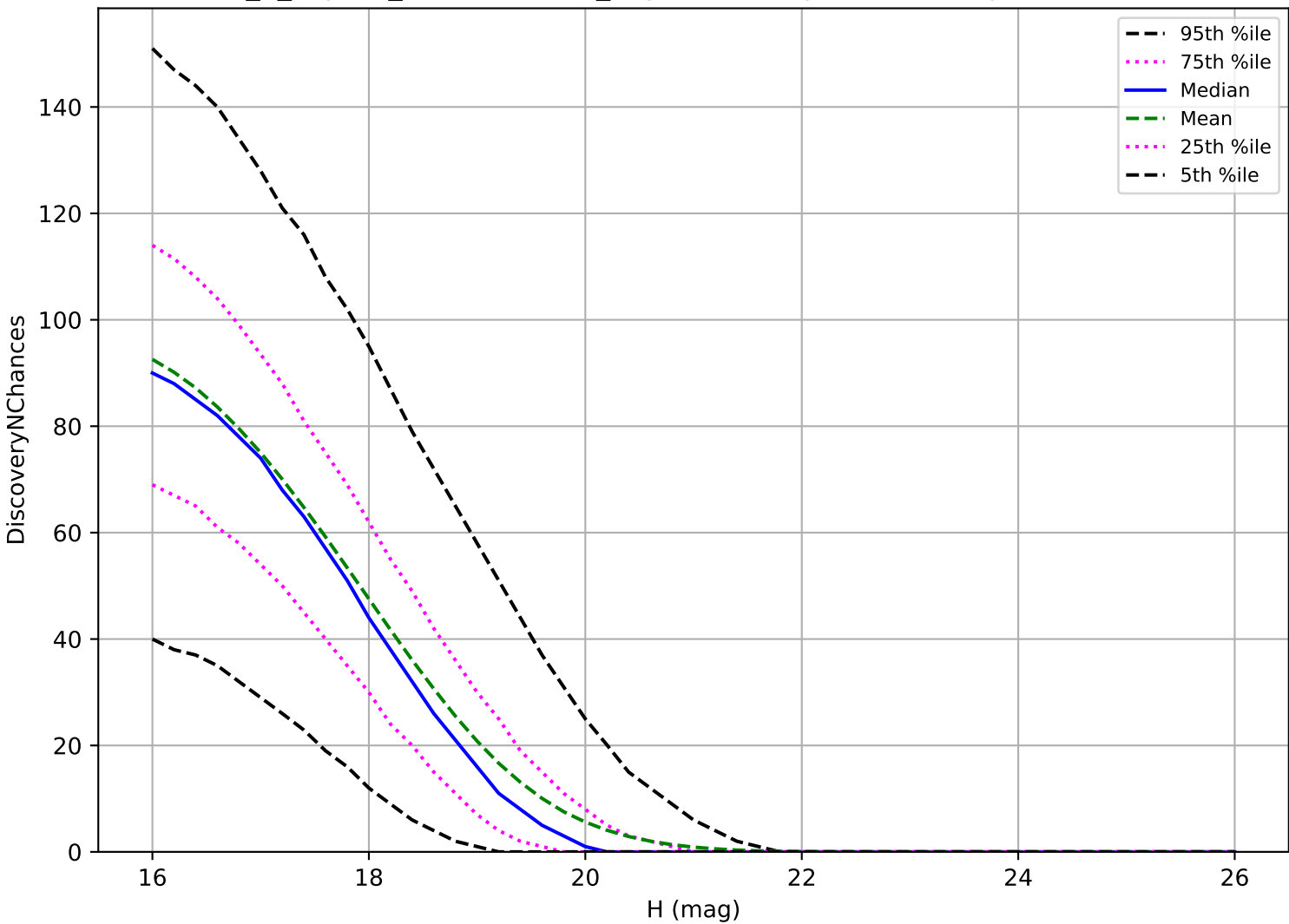
internal_u_expt30_nscale1.2v3.4_10yrs: MBA 3 pairs in 15 nights detection loss
