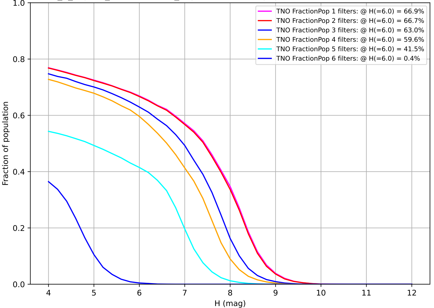
internal_u_expt30_nscale1.2v3.4_10yrs: Fraction of population with colors in X filters TNO
