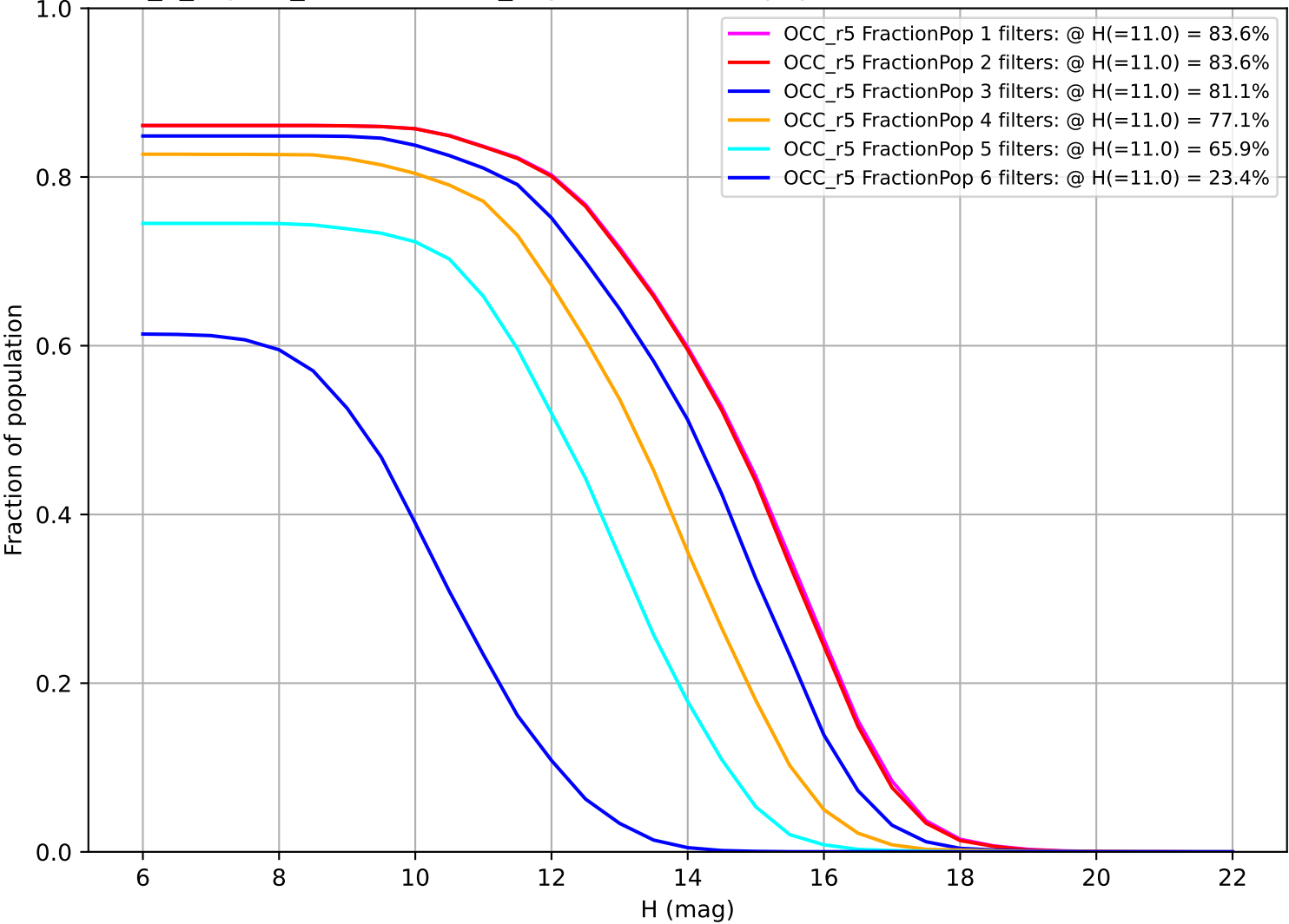
internal_u_expt30_nscale1.2v3.4_10yrs: Fraction of population with colors in X filters OCC_r5
