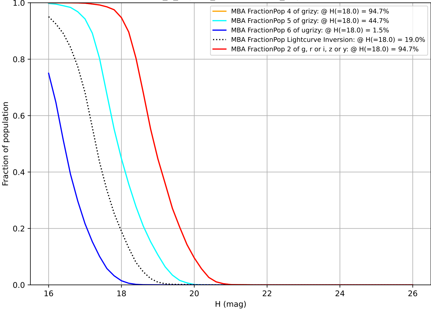
internal_u_expt30_nscale1.2v3.4_10yrs MBA
