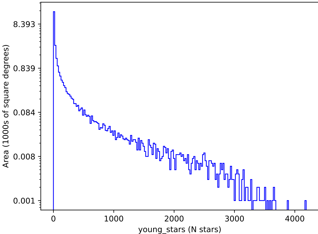
internal_u_expt30_nscale1.2v3.4_10yrs : young_stars
