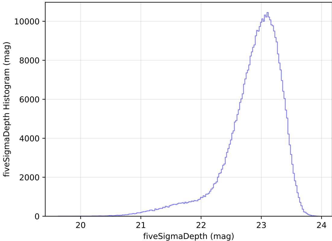
internal_u_expt30_nscale1.2v3.4_10yrs z: fiveSigmaDepth Histogram
