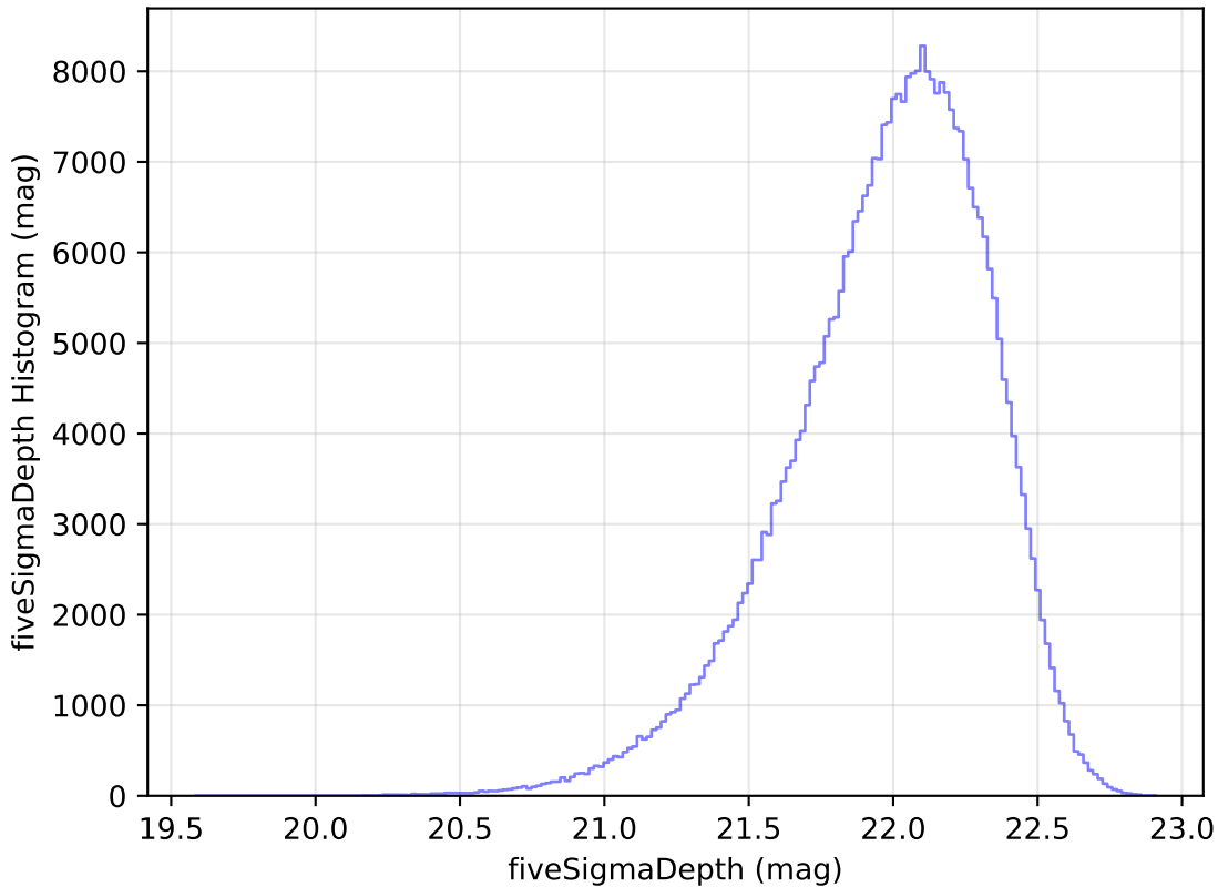
internal_u_expt30_nscale1.2v3.4_10yrs y: fiveSigmaDepth Histogram
