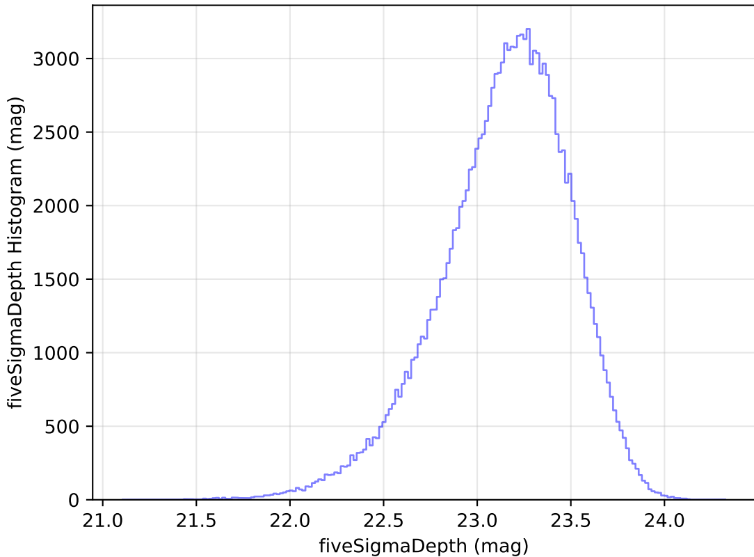
internal_u_expt30_nscale1.2v3.4_10yrs u: fiveSigmaDepth Histogram
