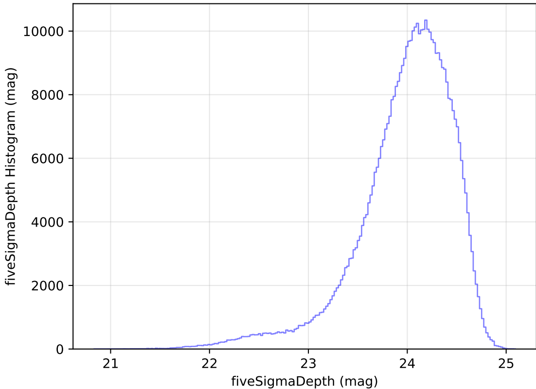
internal_u_expt30_nscale1.2v3.4_10yrs r: fiveSigmaDepth Histogram
