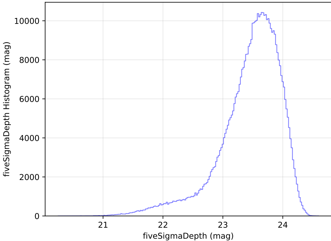
internal_u_expt30_nscale1.2v3.4_10yrs i: fiveSigmaDepth Histogram
