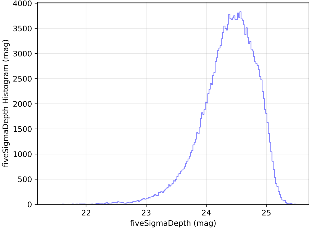
internal_u_expt30_nscale1.2v3.4_10yrs g: fiveSigmaDepth Histogram
