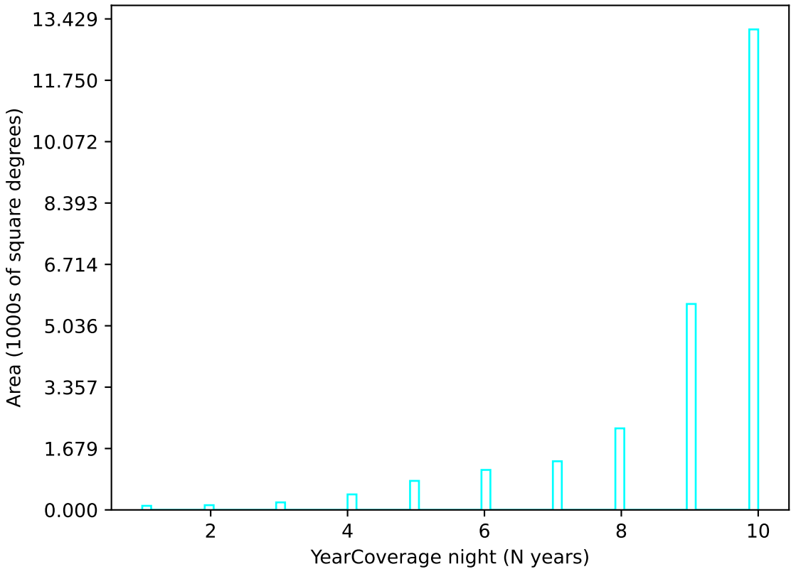
internal_u_expt30_nscale1.2v3.4_10yrs u band: YearCoverage night
