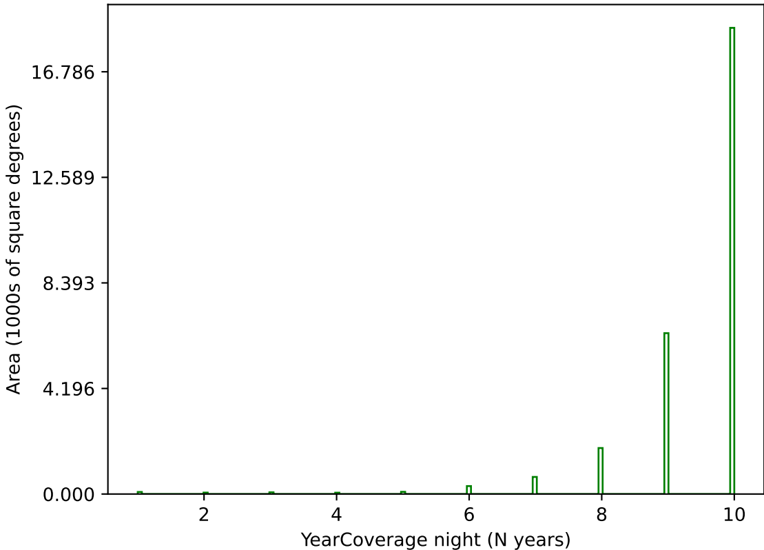
internal_u_expt30_nscale1.2v3.4_10yrs g band: YearCoverage night
