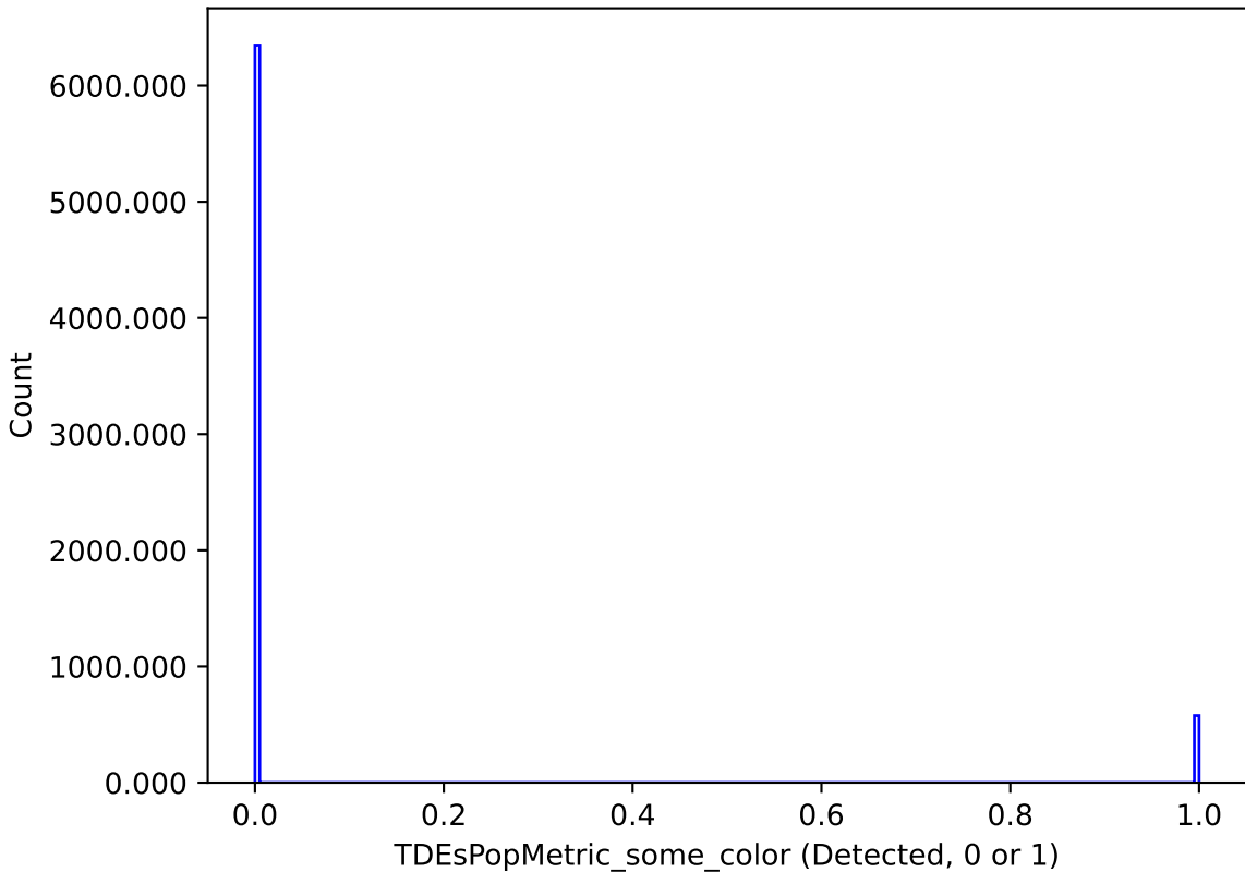
internal_u_expt30_nscale1.2v3.4_10yrs : TDEsPopMetric_some_color
